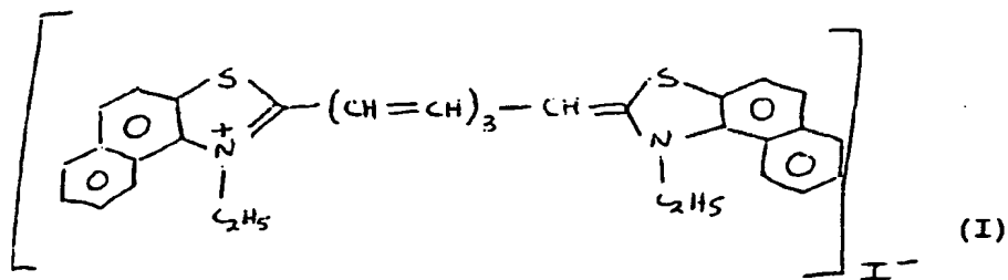
3,3'-diethyl-2,2'-(4,5,4',5'-dibenzo)- thiatricarbocyanine iodide.
